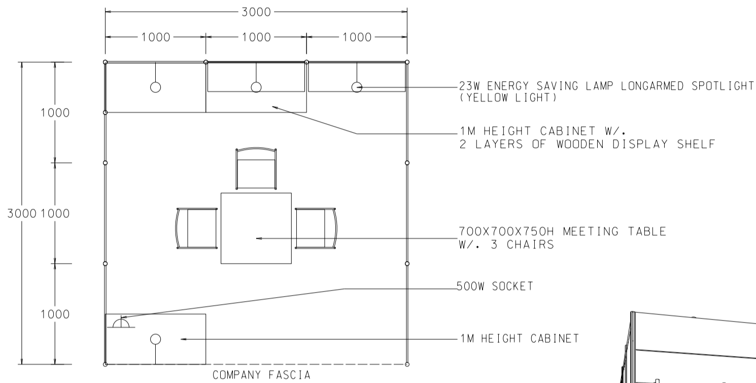
PLAN
