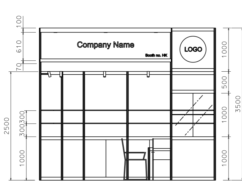
FRONT ELEVATION
